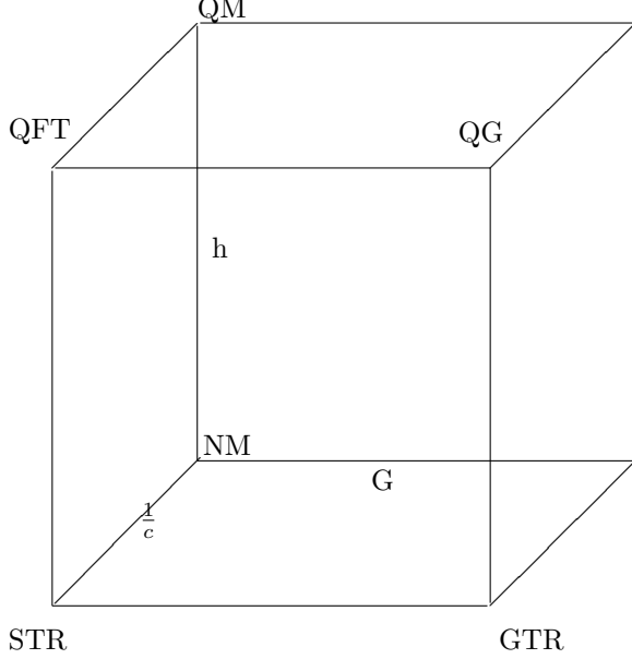
Figure 1: THE MOTION OF AN OBJECT IS DESCRIBED BY NEWTONIAN MECHANICS (NM) AS LONG IT MOVES WITH NON-RELATIVISTIC VELOCITY ( v < c ) AND ITS SIZE IS LARGER THEN \hbar/mc . SPECIAL THEORY OR RELATIVITY (STR) BECOMES IMPORTANT FOR OBJECTS MOVING WITH RELATIVISTIC VELOCITIES. AT SUBATOMIC SCALE GRAVITATIONAL EFFECTS CAN BE IGNORED AND THE SYSTEM IS DESCRIBED BY PURELY QUANTUM MECHANICS (QM). VERY HIGH ENERGETIC PROCESSES AT SUBATOMIC LEVEL ARE DESCRIBED BY QUANTUM FIELD THEORY (QFT) WHICH INCORPORATES STR WITH QM. WE NEED GENERAL THEORY OF RELATIVITY (GTR) WHEN THE SIZE OF A SYSTEM BECOMES COMPARABLE TO \hbar G/c^2 . CLOSE TO THE BIG BANG GRAVITY BECOMES AS STRONG AS ANY OTHER FORCE DESCRIBED BY QUANTUM MECHANICS, SO WE NEED A QUANTUM THEORY OF GRAVITY (QG) THERE.
