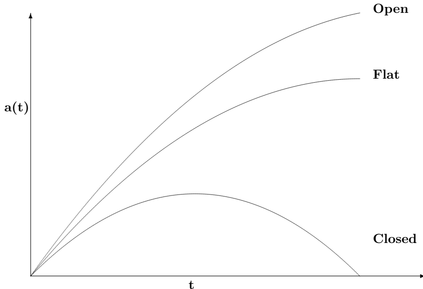
Figure 2: IN A CLOSED MODEL ( \Omega > 1 ) THE UNIVERSE STARTS EXPANDING AT THE BIG BANG AND AFTER REACHING A MAXIMUM SIZE, STARTS COLLAPSING UNTIL THE BIG CRUNCH. IN A FLAT ( \Omega = 1 ) AND OPEN MODEL ( \Omega < 1 ) THE UNIVERSE KEEPS EXPANDING FOREVER.
